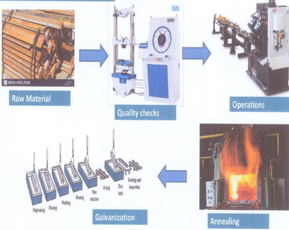
Process flow of Fabrication Section
